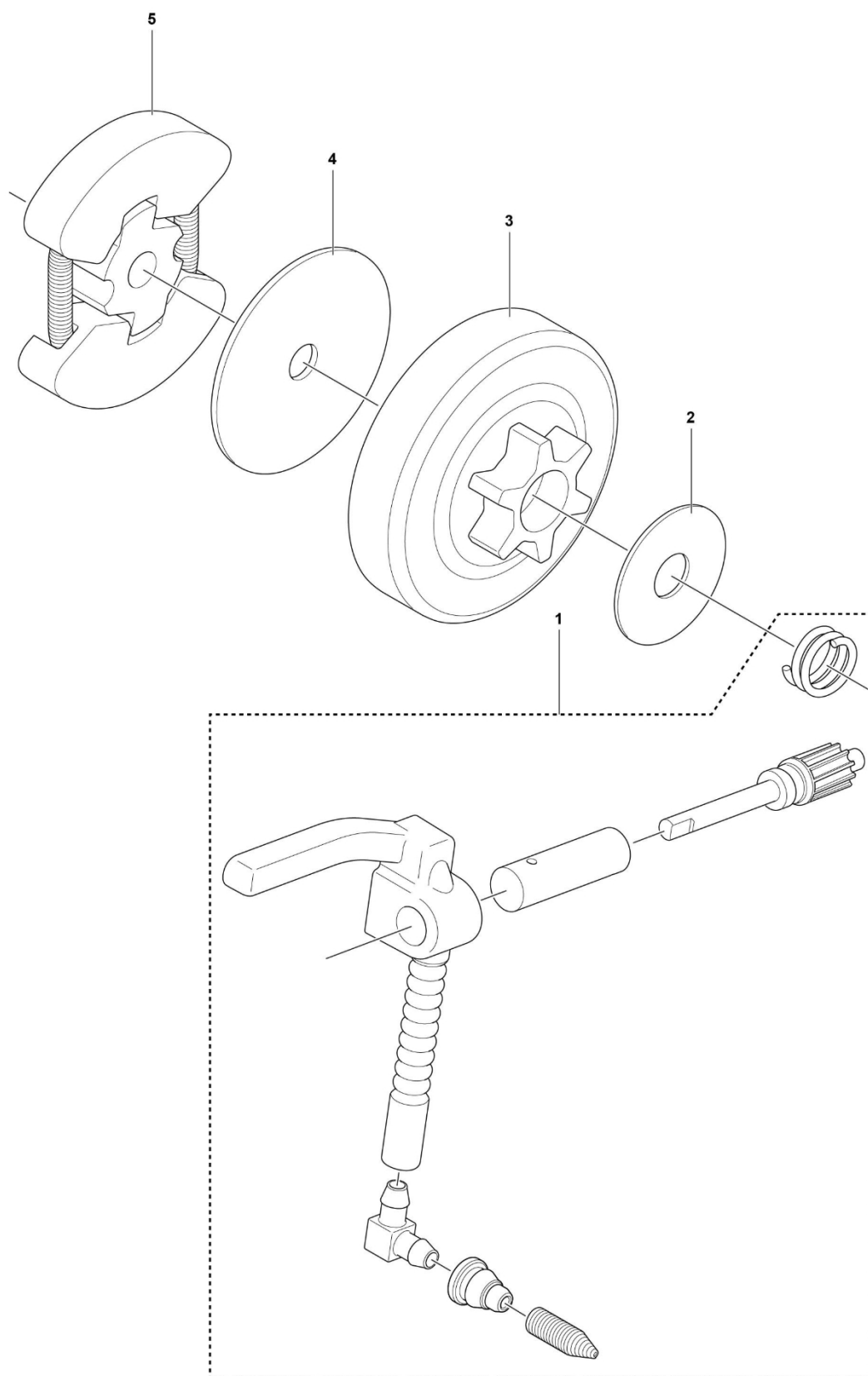
716 CLUTCH AND OIL PUMP
